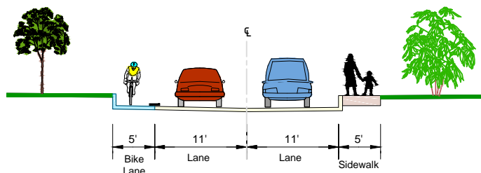
TYPICAL CROSS SECTION N.T.S.
