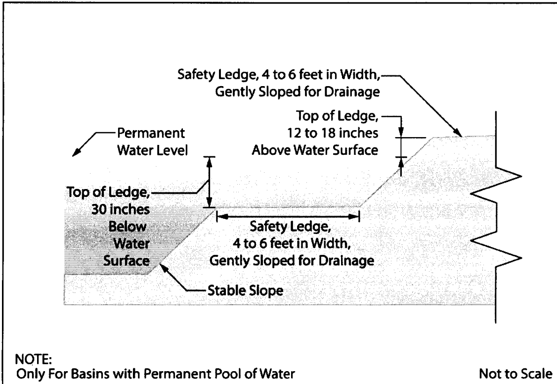
Elevation View –Basin Safety Ledge Configuration
